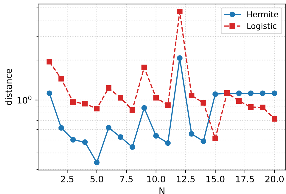
(a) Aitchison distance d_A
