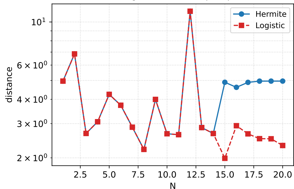
(b) Log-L2 distance d_2(\ln \hat{p}_N, \ln p)
