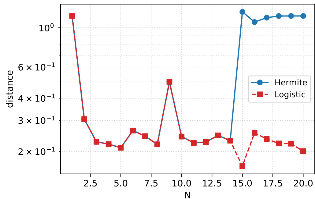
(c) L1 distance d_1
